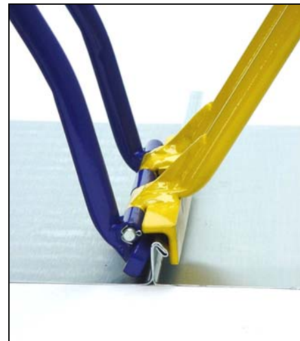
ECO-bender (8520006000)
